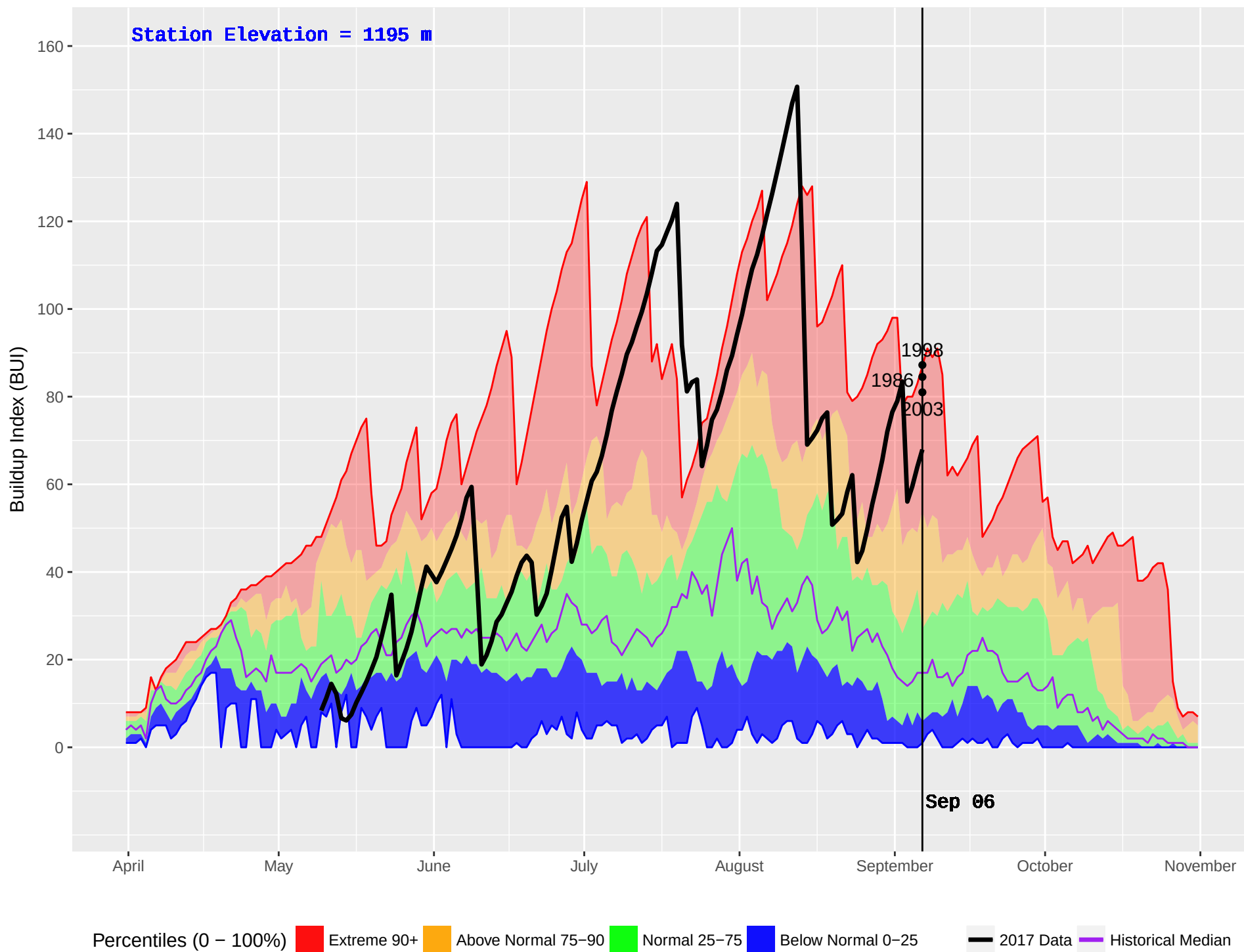
VALEMOUNT 2 (200) : Historical (1986–2016) and Current (2017) Noon Buildup Index (BUI)
