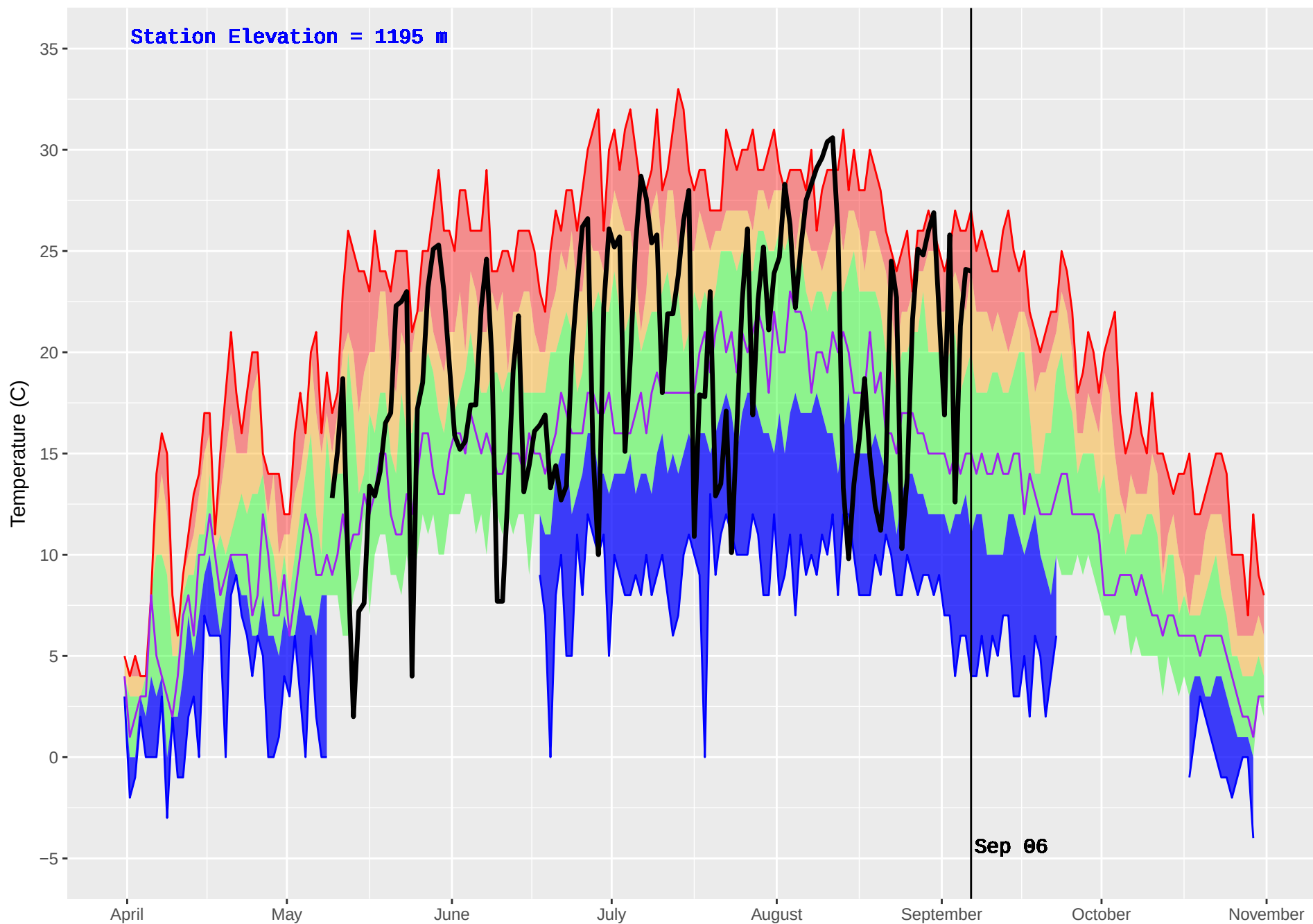
VALEMOUNT 2 (200) : Historical (1986–2016) and Current (2017) Noon Temperature
